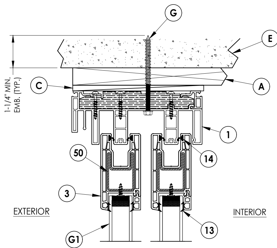
2 3 VERTICAL CROSS SECTION Shown w/ 1X Buck
