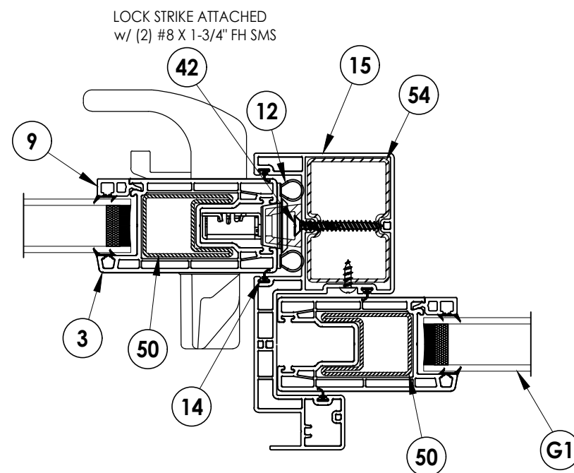
2 HORIZONTAL CROSS SECTION Shown w/ 1X Buck (Direct to Masonry Similar)
