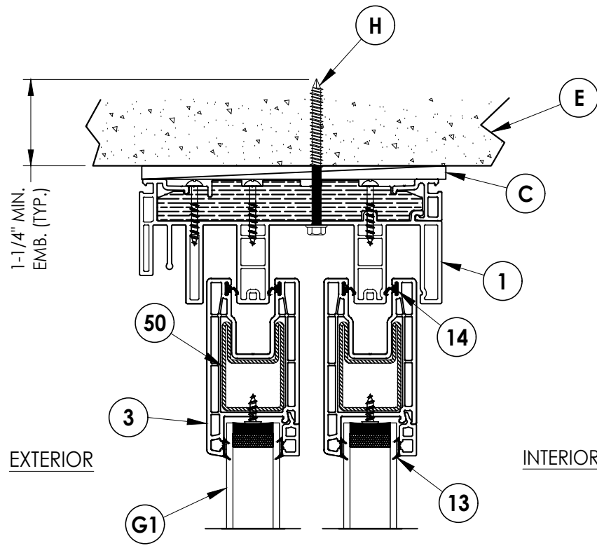
3 3 VERTICAL CROSS SECTION Shown Direct to Masonry
