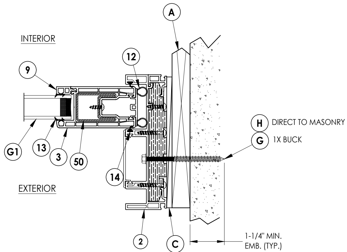
2 HORIZONTAL CROSS SECTION Shown w/ 1X Buck (Direct to Masonry Similar)
